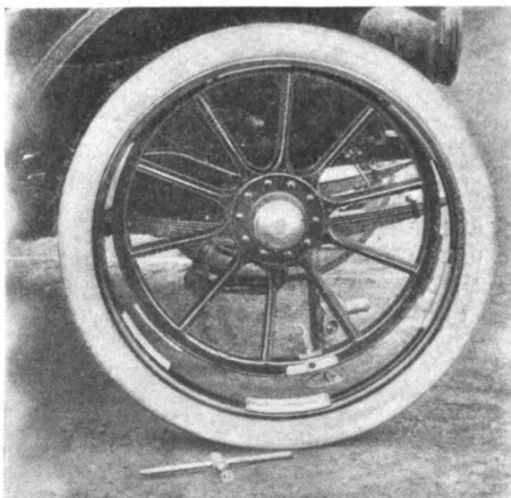
Dow Rim With Tire In Place Ready to Slip Over.
